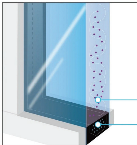
ARGON GAS
